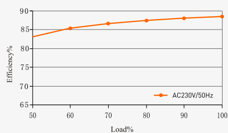
YSD-300WHC-24
