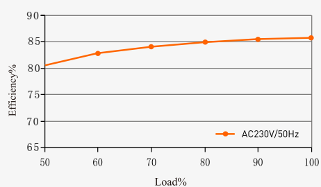
YSD-300WHC-12
